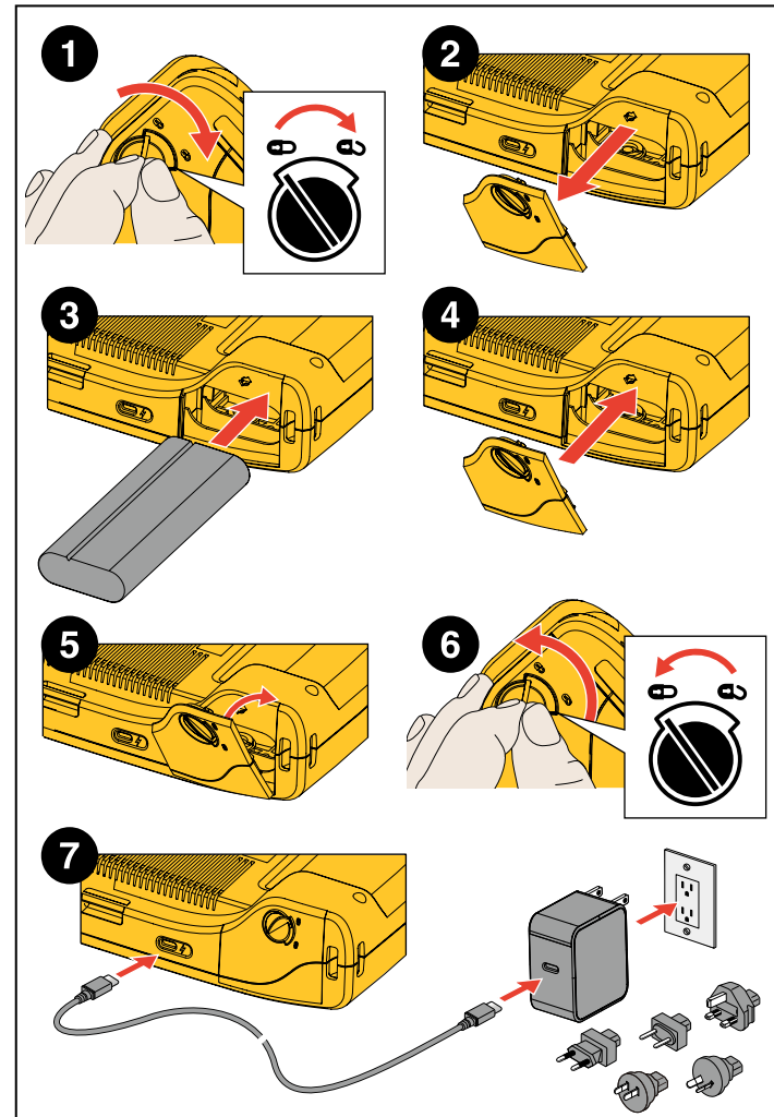
Figure 1. Battery
