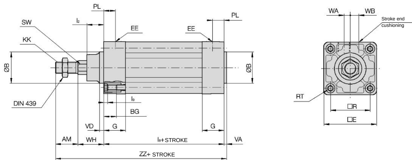
CP95K□BØ-Stroke
