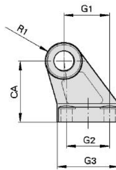
Mounting type E
