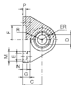
Mounting type CR Rear clevis with ball joint
