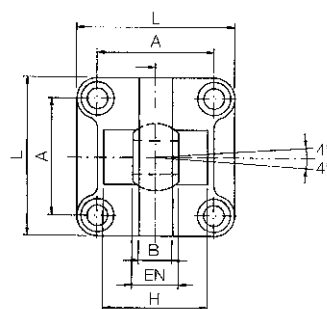
Mounting type CR Rear clevis with ball joint
