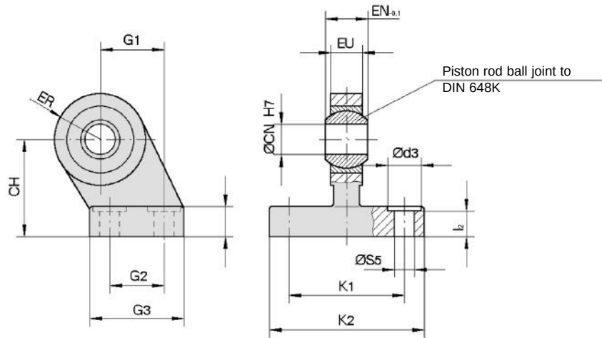
Mounting type ES
