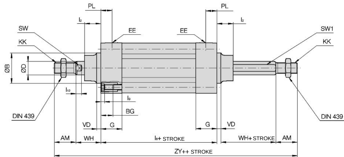
CP95K□BØ-Stroke W
