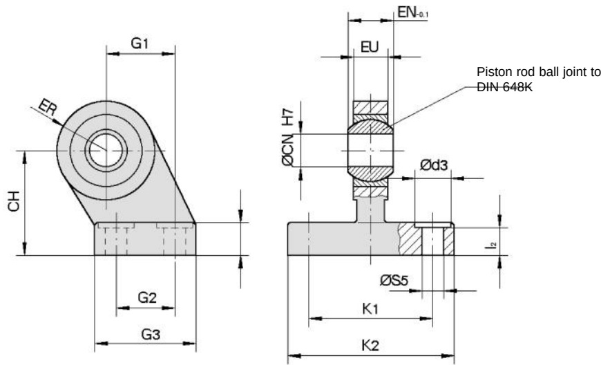
Mounting type ES
