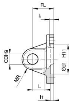
Mounting type C
