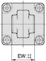
Mounting type C
